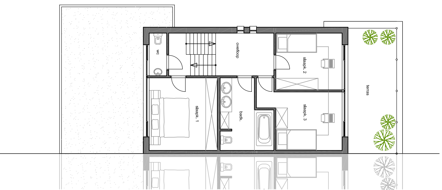
Blok C, woning 1: Plan verdieping
